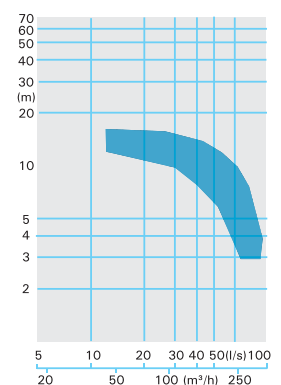
VX 34... -6 pole
