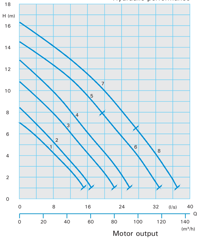
Hydraulic performance
