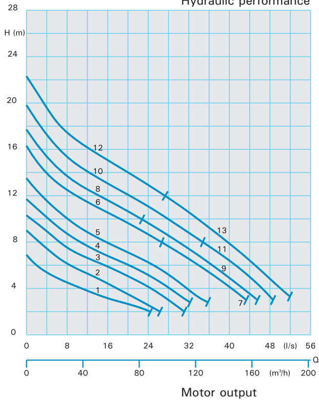
Hydraulic performance
